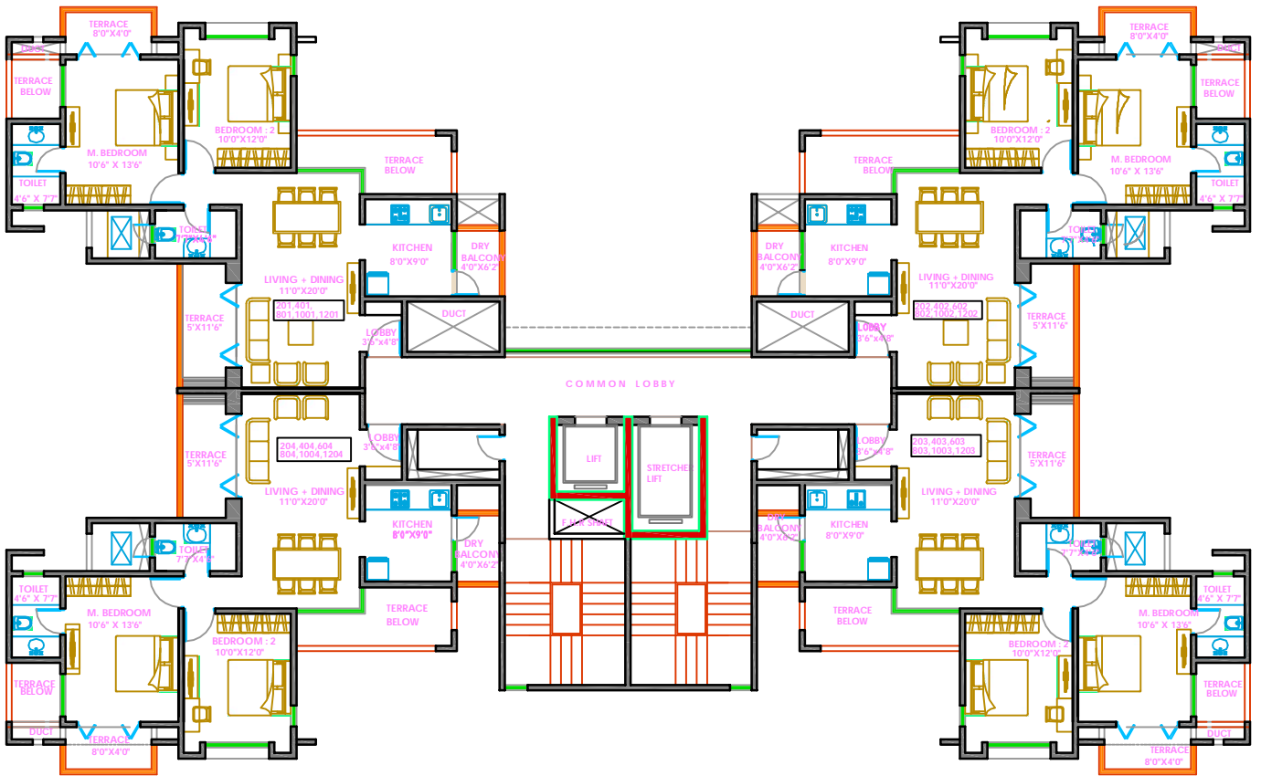
TYP.EVEN FLOOR LVL PLAN
